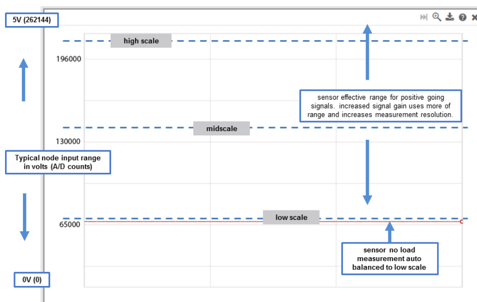
Figure 52 - Differential Input Resolution and Offset (18-bit Node)
