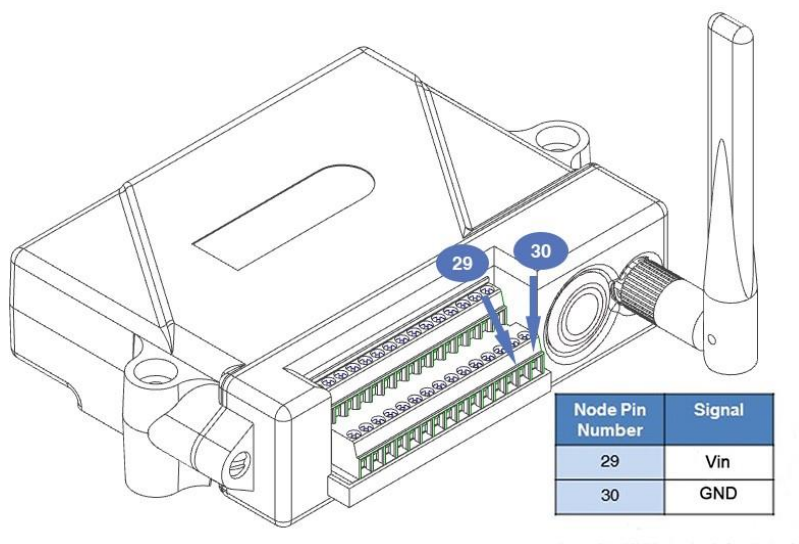
Figure 53 - External Power Connection
